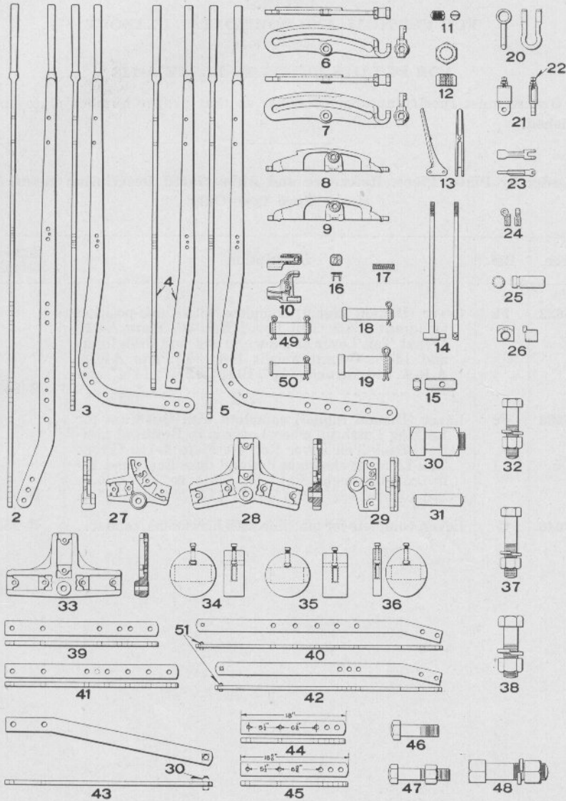
DETAILS OF LEVERS FOR S. & F. MACHINE
